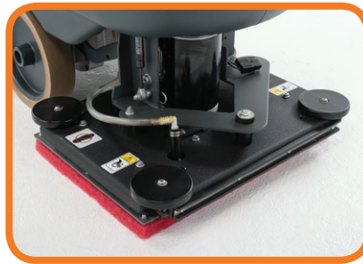
Orbital cleaning
